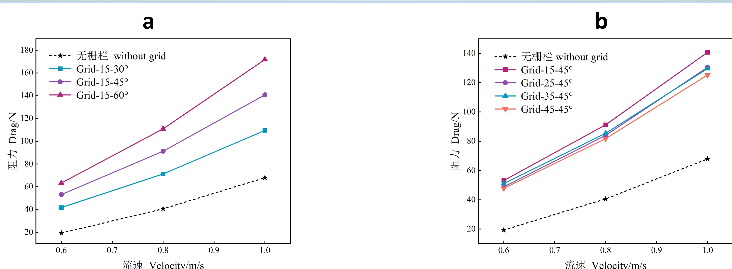
Fig.1 a) Variation of cod-end drag with flow velocity at different inclination angles. b) Variation of cod-end drag with flow velocity at different grid bar spacings.
