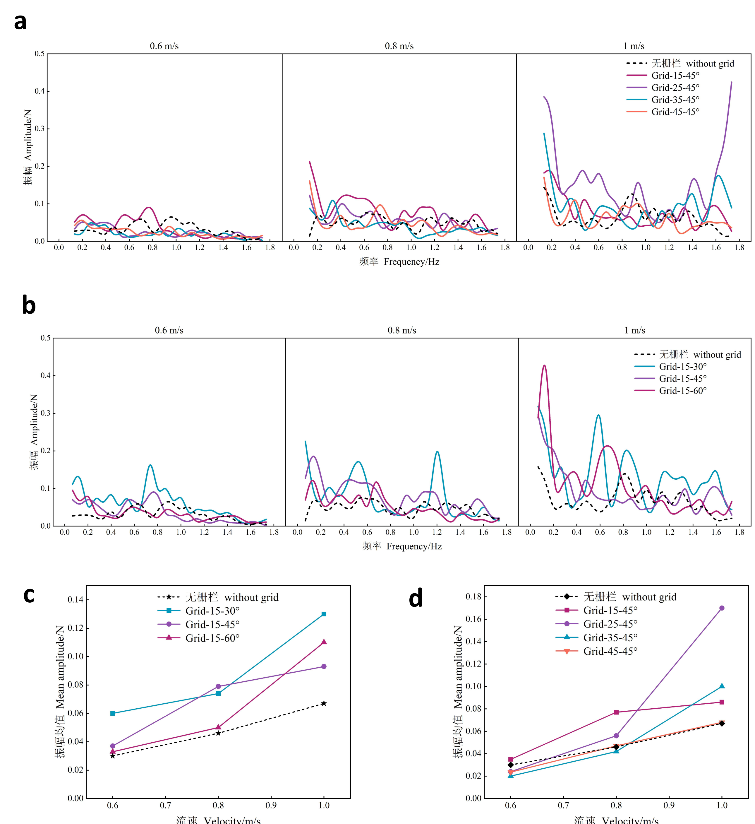
Fig.3 a) Drag amplitude of cod-end structure at different bar spacings. b) Drag amplitude of cod-end structure at different inclination angles. c) Variation of average drag amplitude of the cod-end structure with different Inclination Angles. d) Variation of average drag amplitude of the cod-end structure with different grid bar spacings.
