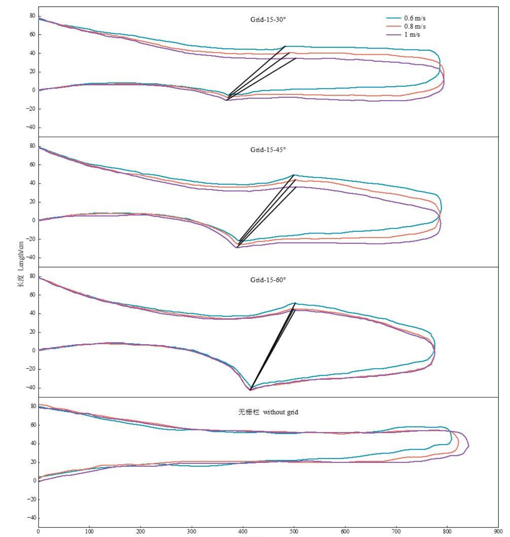
Fig.2 The shape of the cod-end with flow velocity at different inclination angles.
